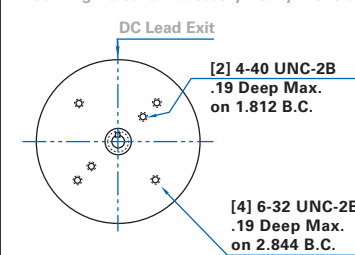
33A, 42A Motors/Gearmotors Mounting Holes for Accessory Ready Models
